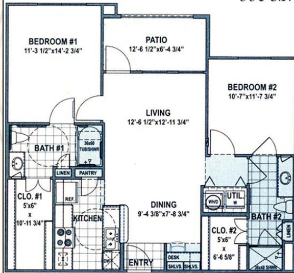
B-1 Two Bedroom / Two Bath 990 S.F.
